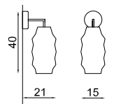
M155/A1/LU H 40 cm - Sp 21 cm L 15 cm E27 1x60W Max
