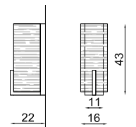
M153/A1/NL H 43 cm - Sp 22 cm L 16 cm E27 1x60W Max
