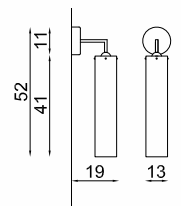
M160/A1/NL H 52 cm - Sp 19 cm L 13 cm E27 1x60W Max
